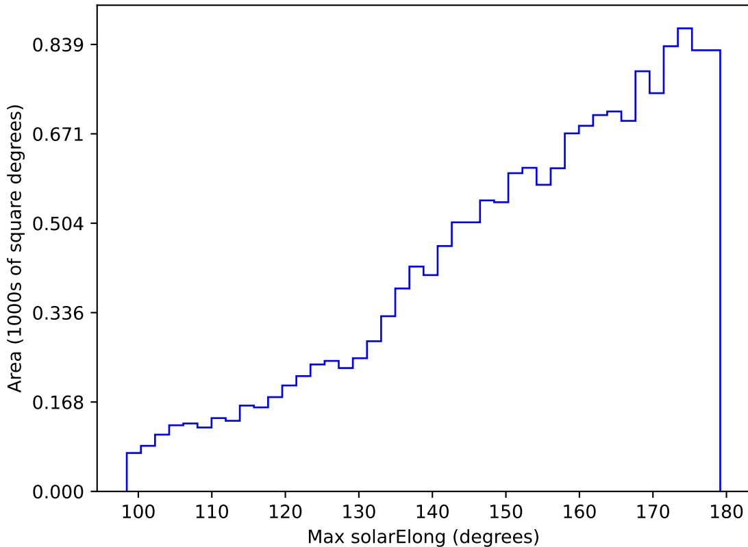
smc_lmc_v3.3_10yrs WFD g band: Max solarElong
