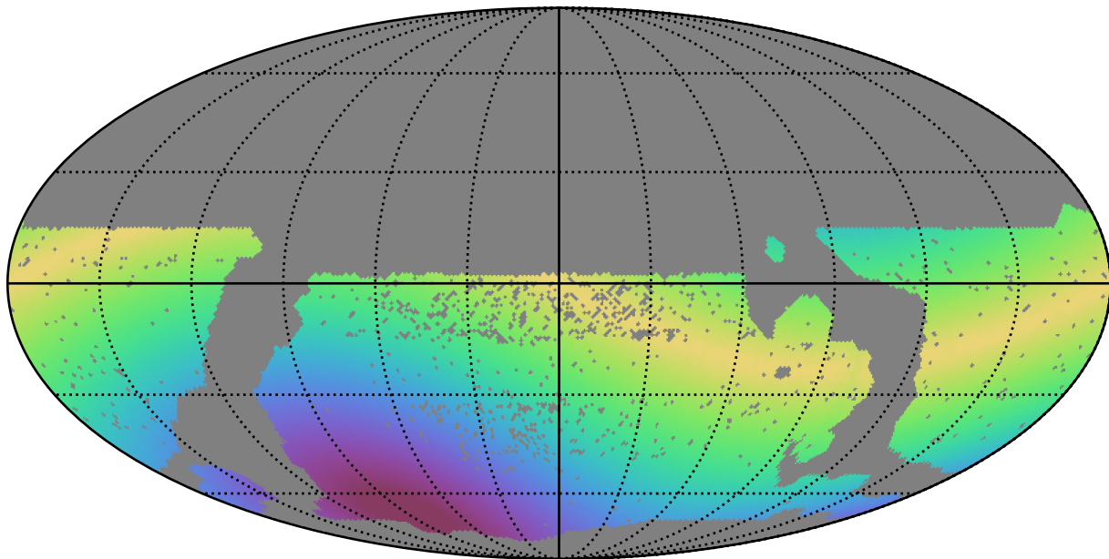
smc_lmc_v3.3_10yrs WFD all bands: Max solarElong
