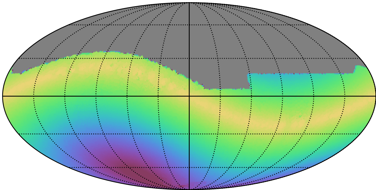
smc_lmc_v3.3_10yrs All sky z band: Max solarElong
