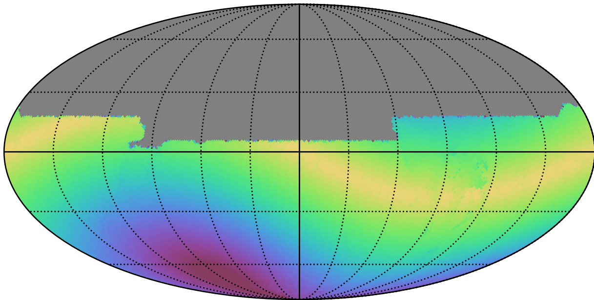
smc_lmc_v3.3_10yrs All sky y band: Max solarElong
