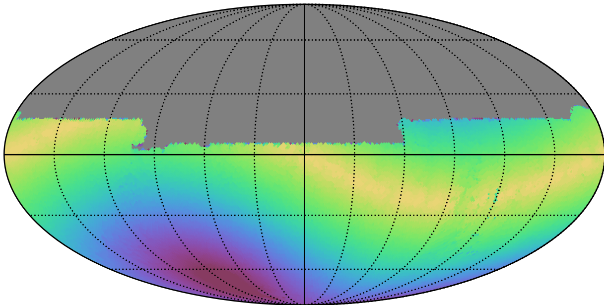
smc_lmc_v3.3_10yrs All sky u band: Max solarElong
