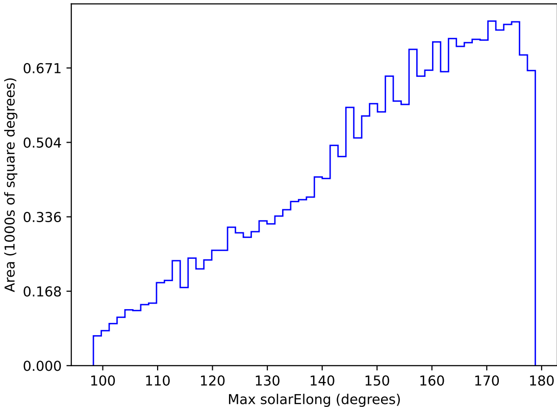
smc_lmc_v3.3_10yrs All sky u band: Max solarElong
