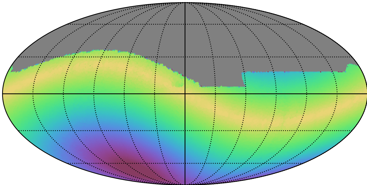
smc_lmc_v3.3_10yrs All sky r band: Max solarElong
