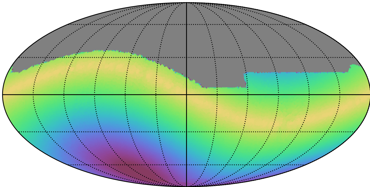
smc_lmc_v3.3_10yrs All sky i band: Max solarElong
