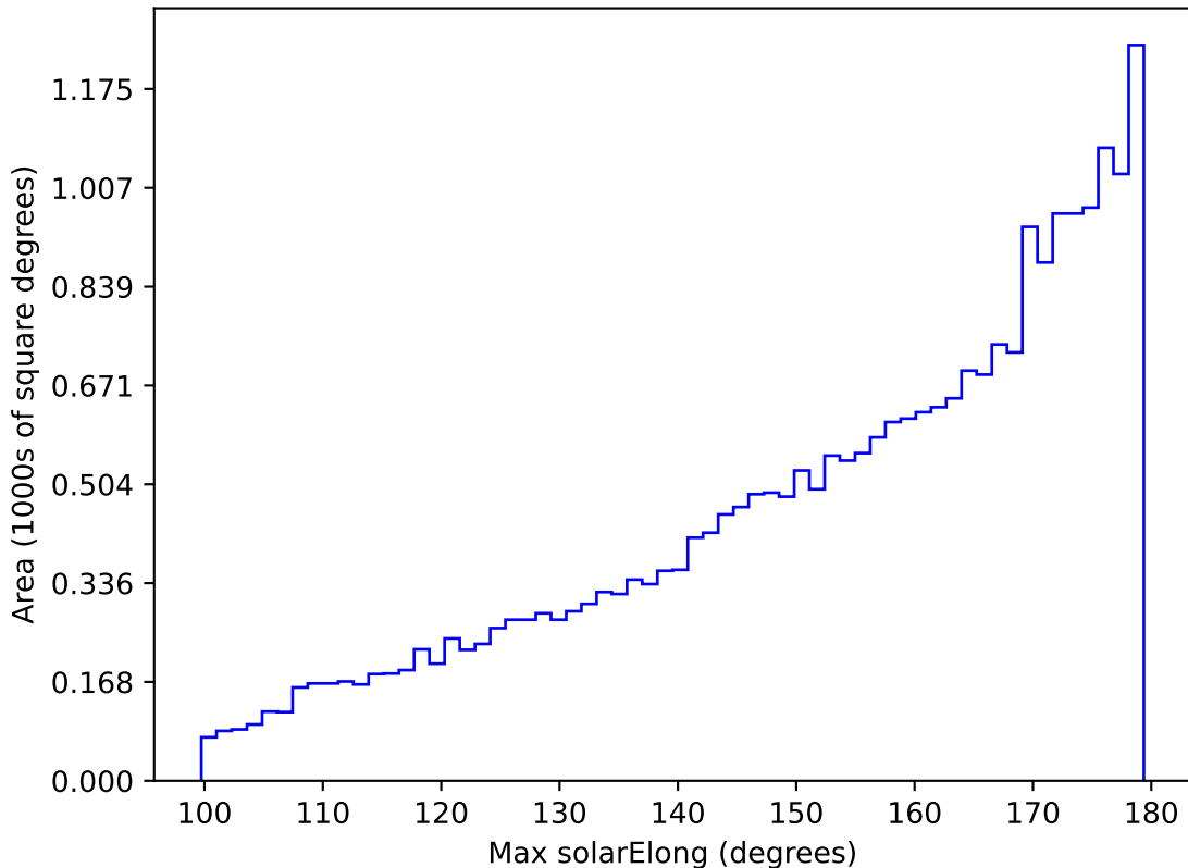
smc_lmc_v3.3_10yrs All sky i band: Max solarElong
