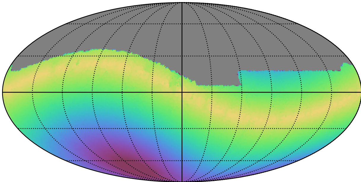
smc_lmc_v3.3_10yrs All sky g band: Max solarElong
