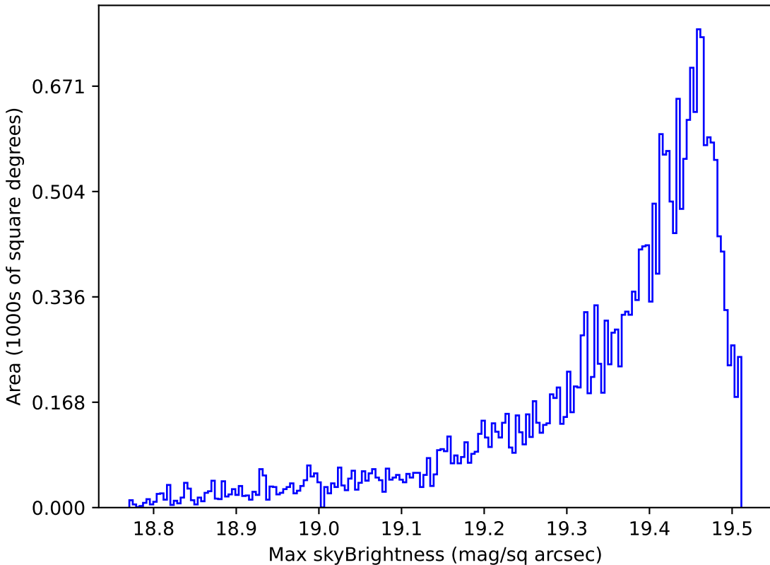
smc_lmc_v3.3_10yrs Yr 1 z band: Max skyBrightness
