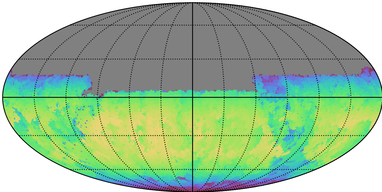
smc_lmc_v3.3_10yrs Yr 1 y band: Max skyBrightness
