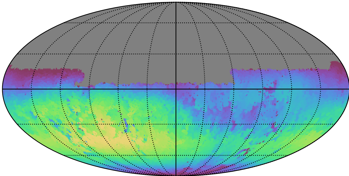
smc_lmc_v3.3_10yrs Yr 1 u band: Max skyBrightness
