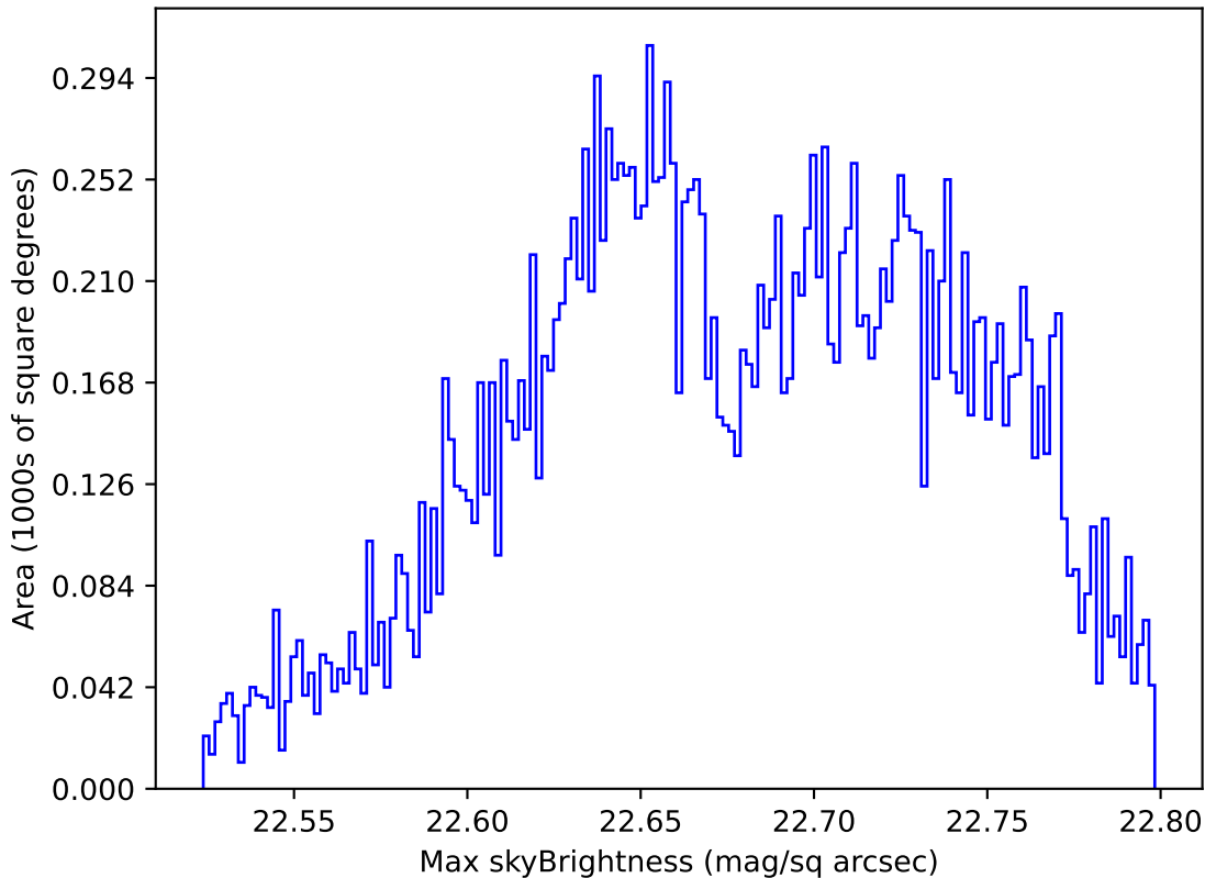
smc_lmc_v3.3_10yrs Yr 1 u band: Max skyBrightness
