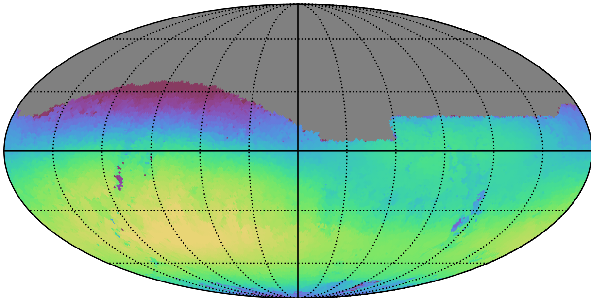
smc_lmc_v3.3_10yrs Yr 1 r band: Max skyBrightness
