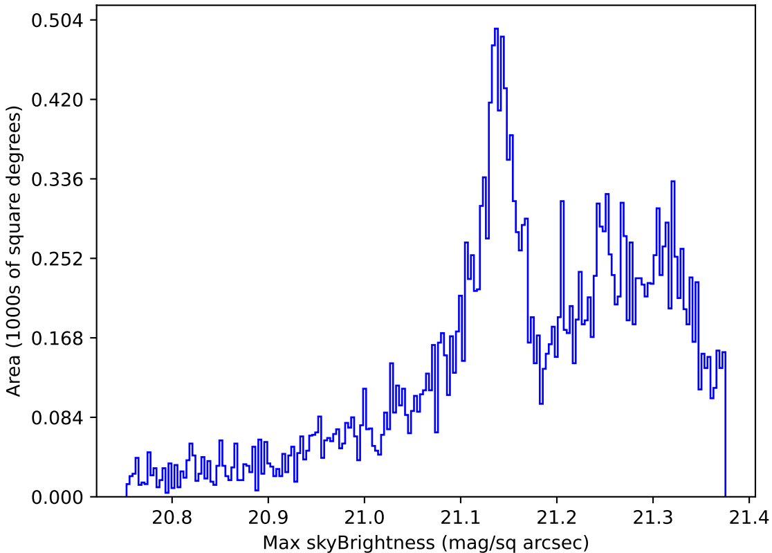
smc_lmc_v3.3_10yrs Yr 1 r band: Max skyBrightness
