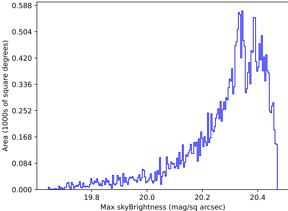
smc_lmc_v3.3_10yrs Yr 1 i band: Max skyBrightness
