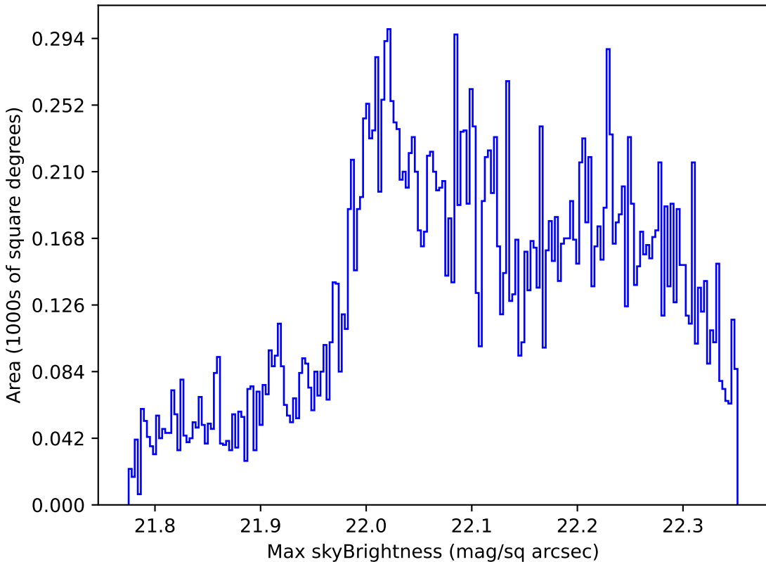
smc_lmc_v3.3_10yrs Yr 1 g band: Max skyBrightness
