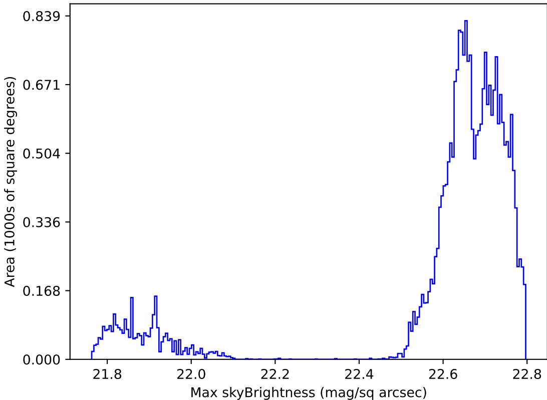
smc_lmc_v3.3_10yrs Yr 1 all bands: Max skyBrightness
