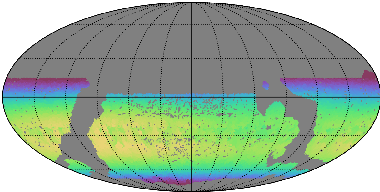
smc_lmc_v3.3_10yrs WFD z band: Max skyBrightness
