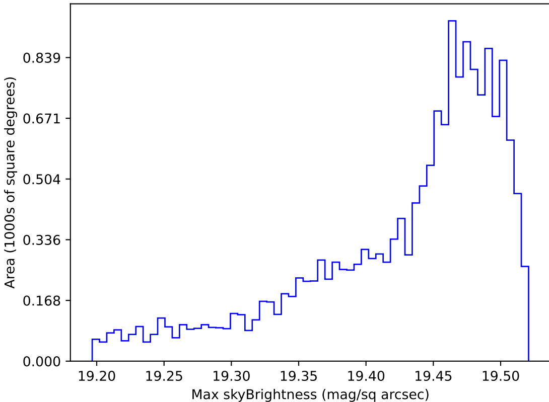
smc_lmc_v3.3_10yrs WFD z band: Max skyBrightness
