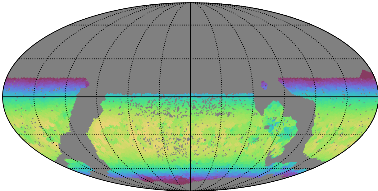
smc_lmc_v3.3_10yrs WFD y band: Max skyBrightness
