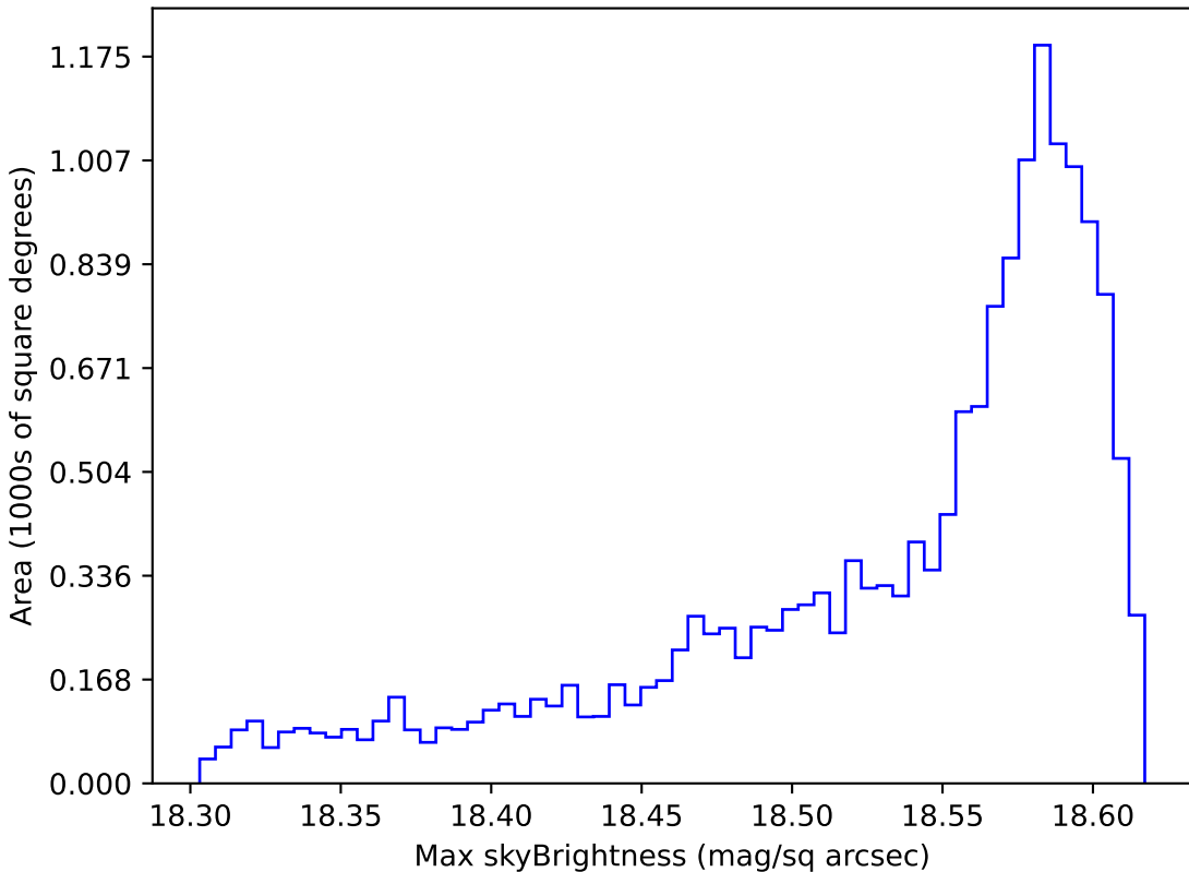
smc_lmc_v3.3_10yrs WFD y band: Max skyBrightness
