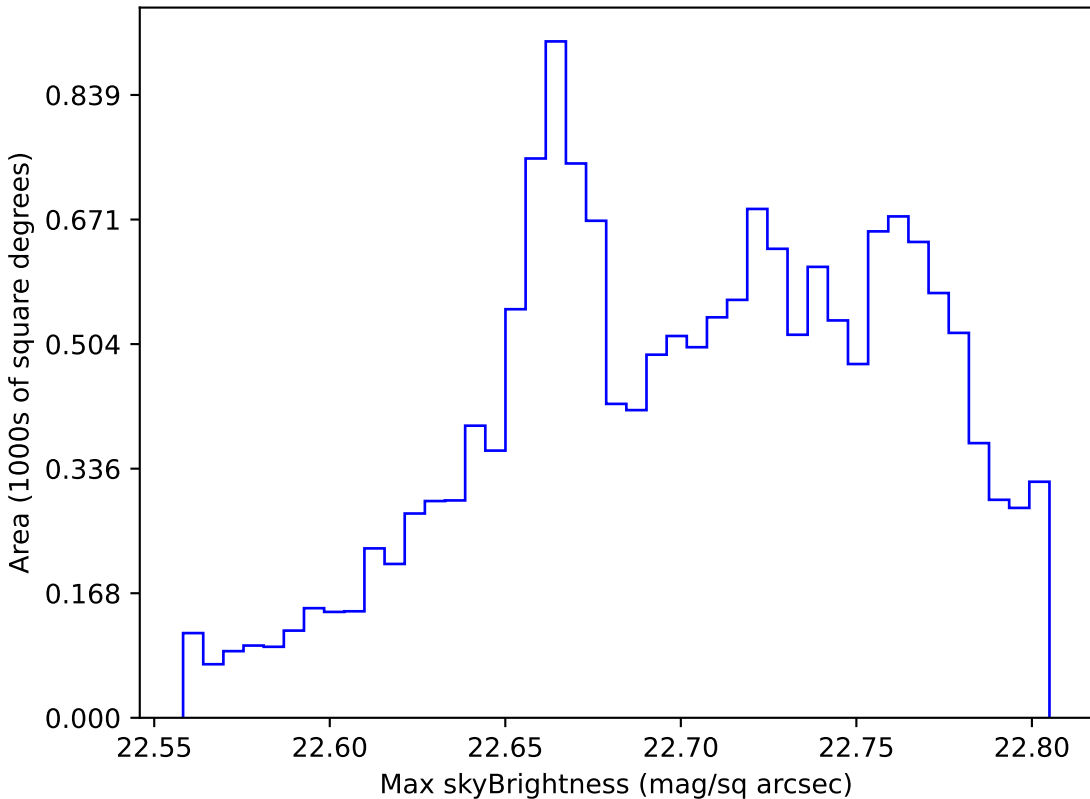
smc_lmc_v3.3_10yrs WFD u band: Max skyBrightness
