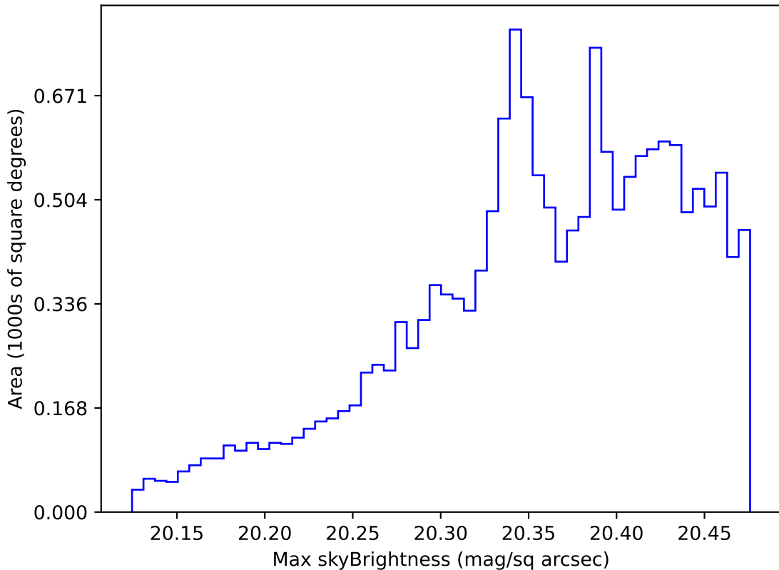
smc_lmc_v3.3_10yrs WFD i band: Max skyBrightness
