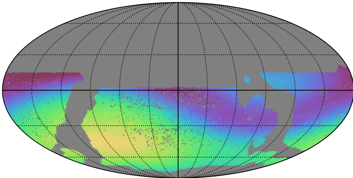
smc_lmc_v3.3_10yrs WFD g band: Max skyBrightness
