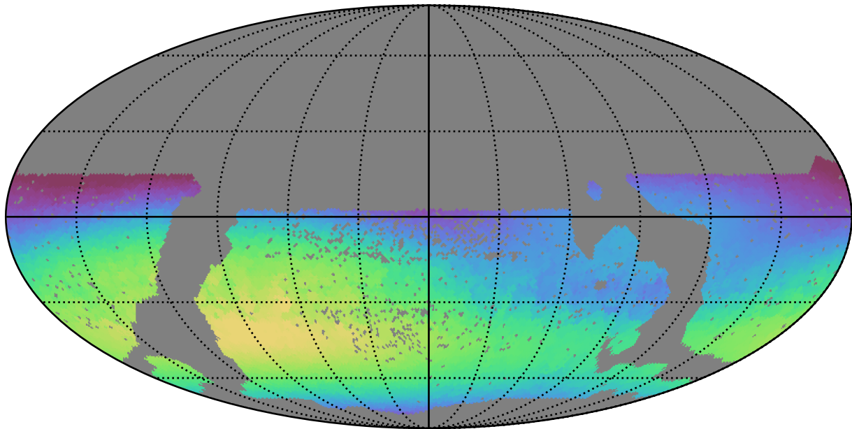
smc_lmc_v3.3_10yrs WFD all bands: Max skyBrightness
