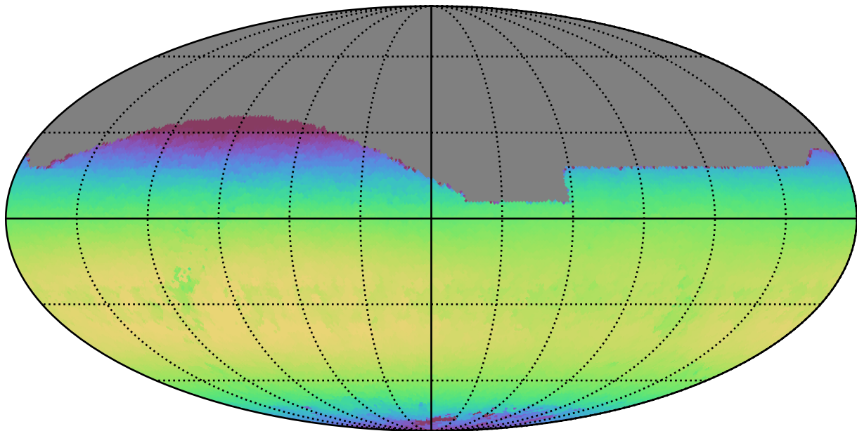
smc_lmc_v3.3_10yrs All sky z band: Max skyBrightness
