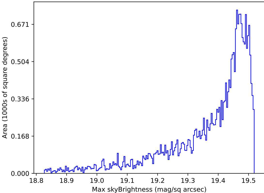
smc_lmc_v3.3_10yrs All sky z band: Max skyBrightness
