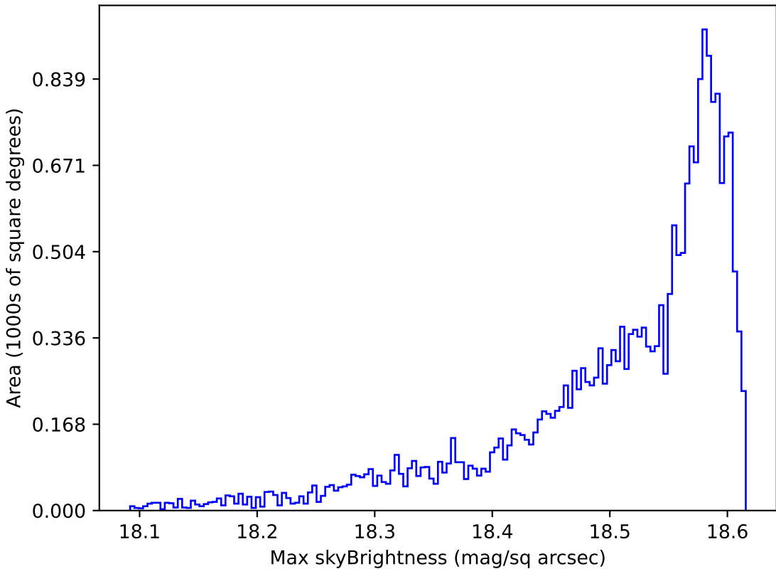
smc_lmc_v3.3_10yrs All sky y band: Max skyBrightness
