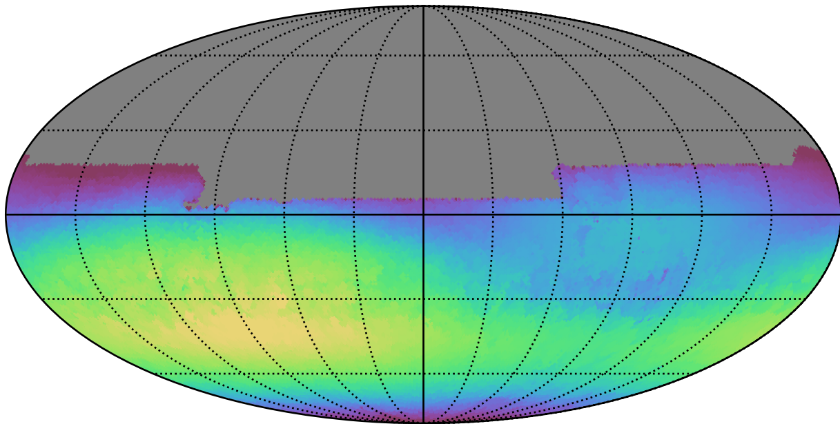
smc_lmc_v3.3_10yrs All sky u band: Max skyBrightness
