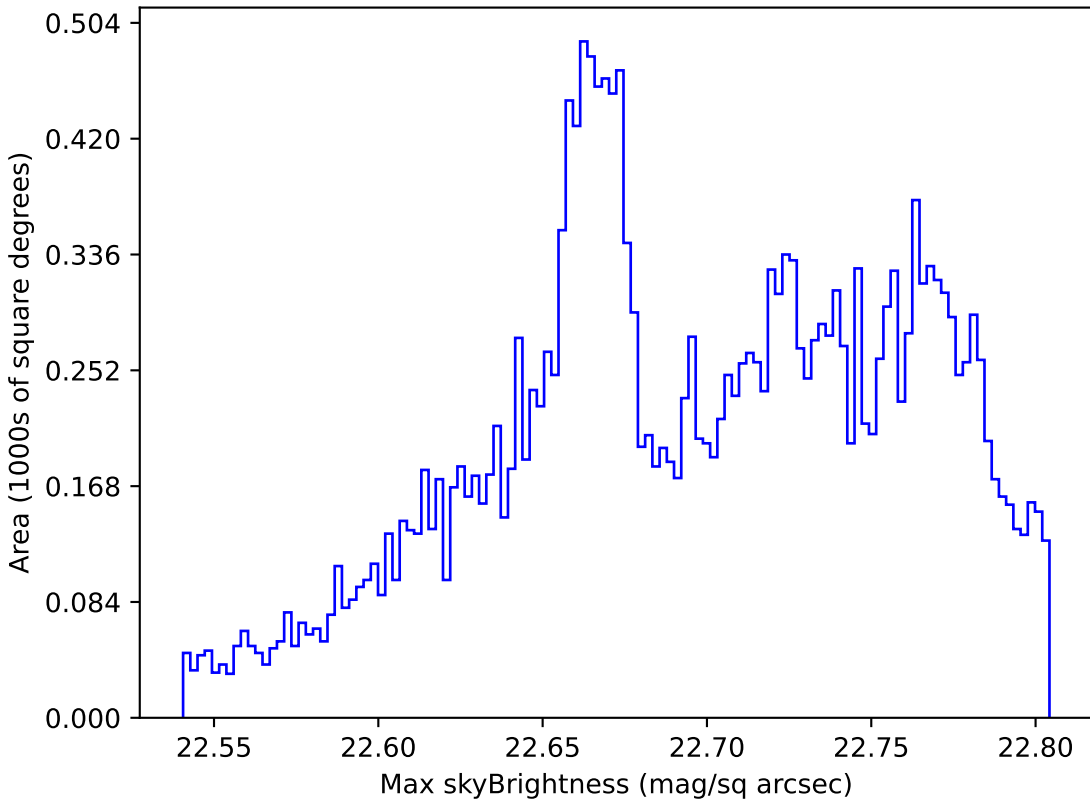
smc_lmc_v3.3_10yrs All sky u band: Max skyBrightness
