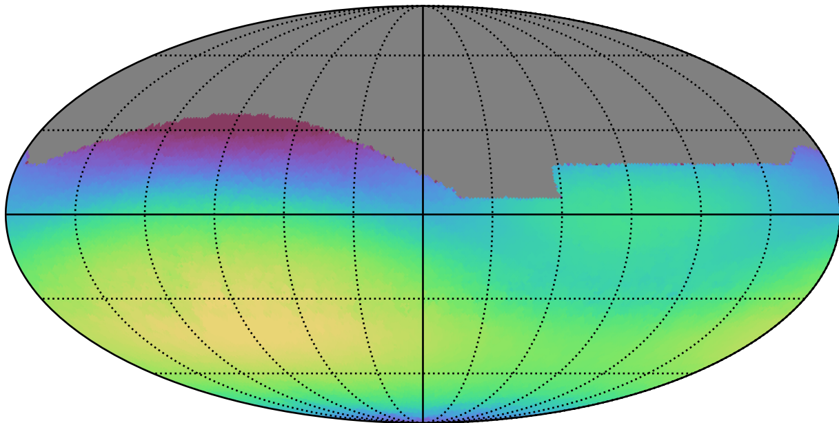
smc_lmc_v3.3_10yrs All sky r band: Max skyBrightness
