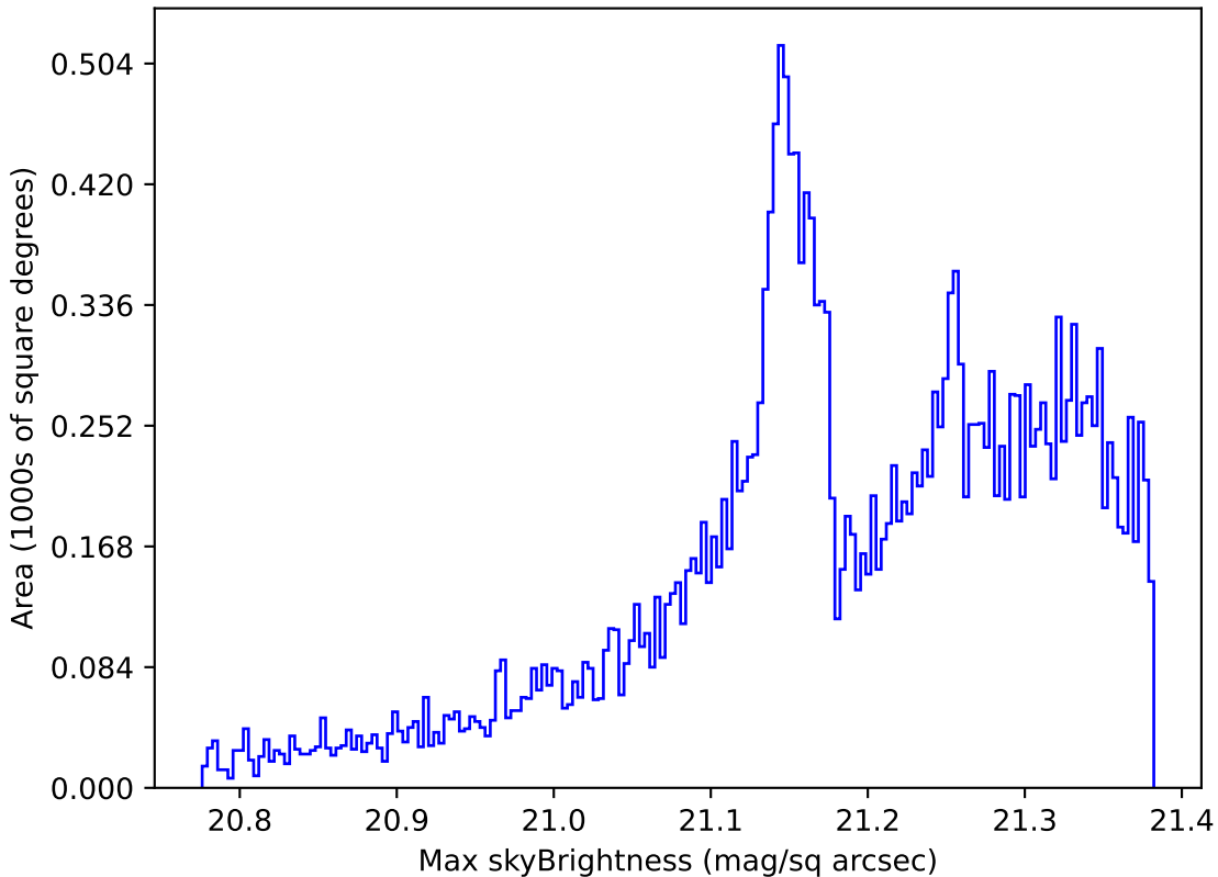
smc_lmc_v3.3_10yrs All sky r band: Max skyBrightness
