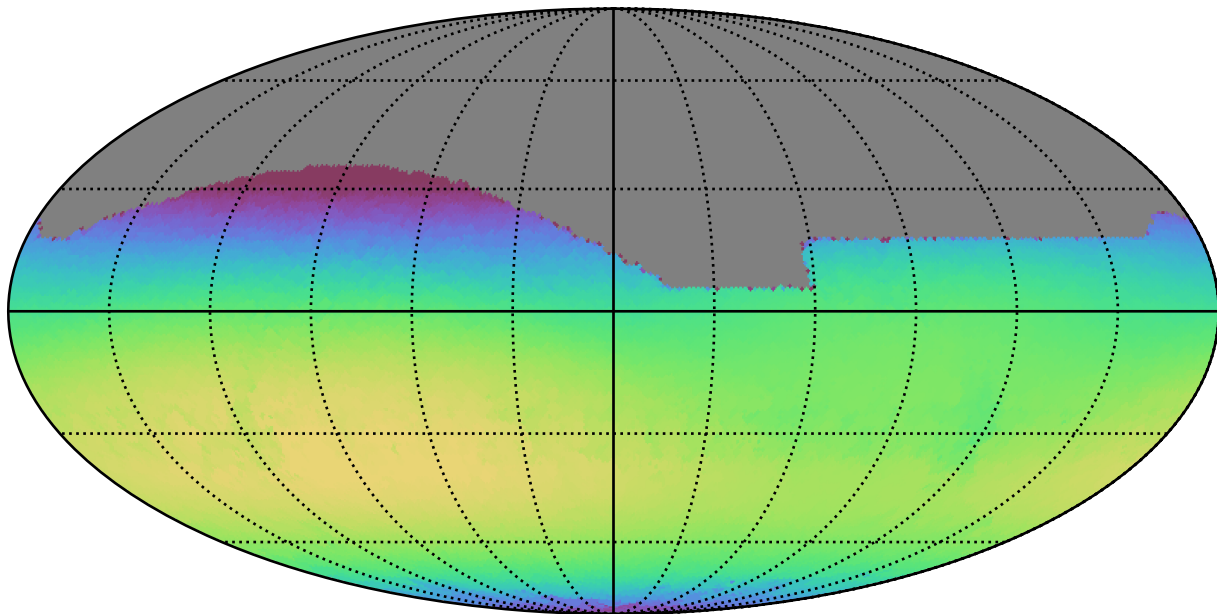
smc_lmc_v3.3_10yrs All sky i band: Max skyBrightness
