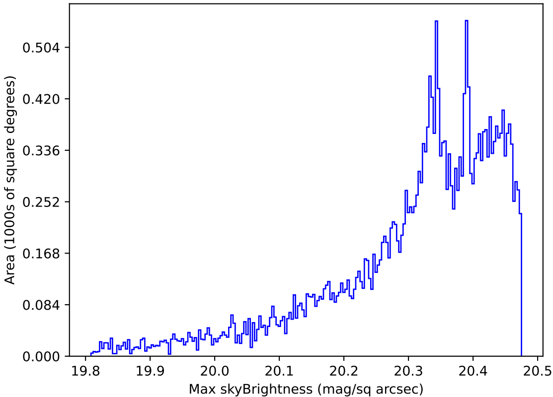
smc_lmc_v3.3_10yrs All sky i band: Max skyBrightness
