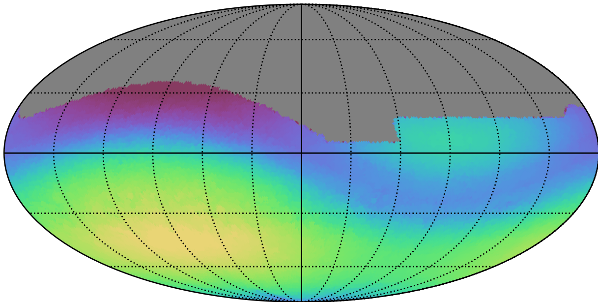
smc_lmc_v3.3_10yrs All sky g band: Max skyBrightness
