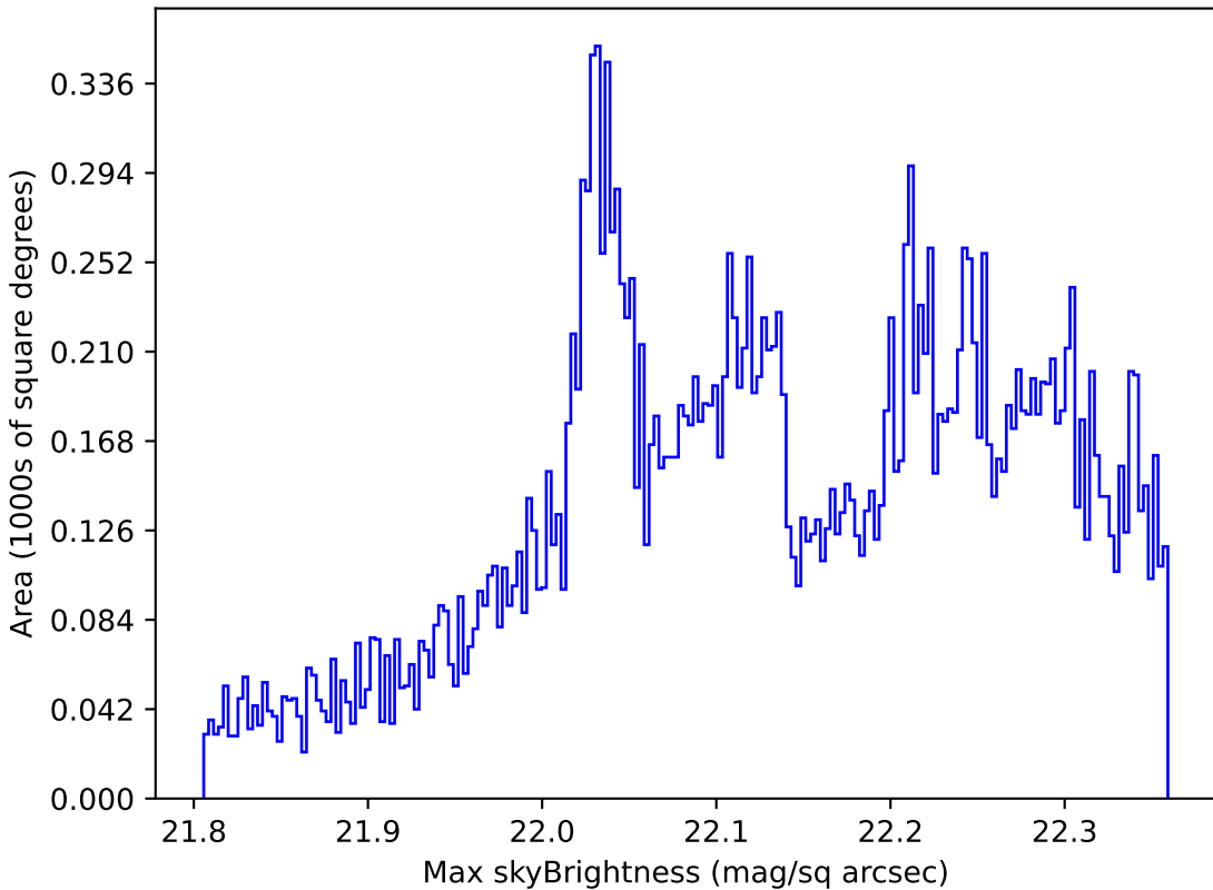
smc_lmc_v3.3_10yrs All sky g band: Max skyBrightness
