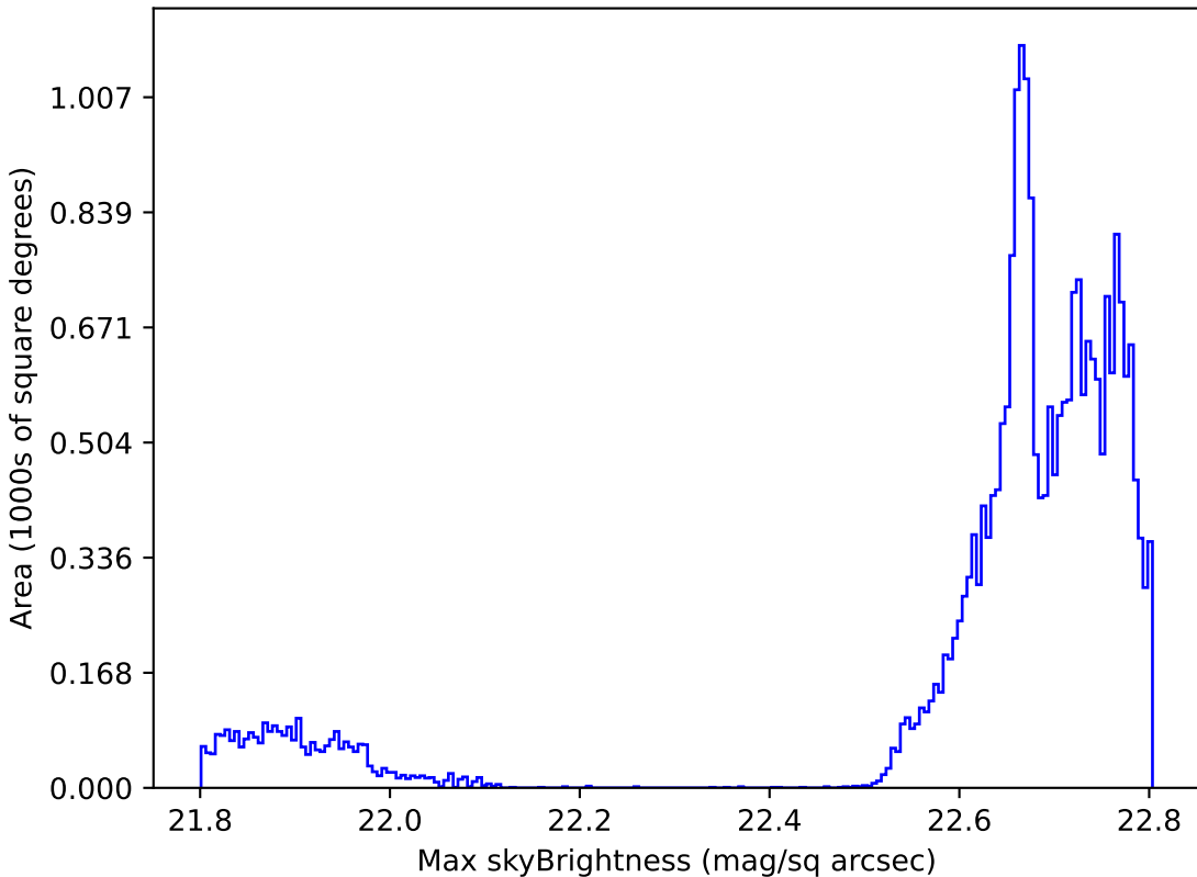
smc_lmc_v3.3_10yrs All sky all bands: Max skyBrightness
