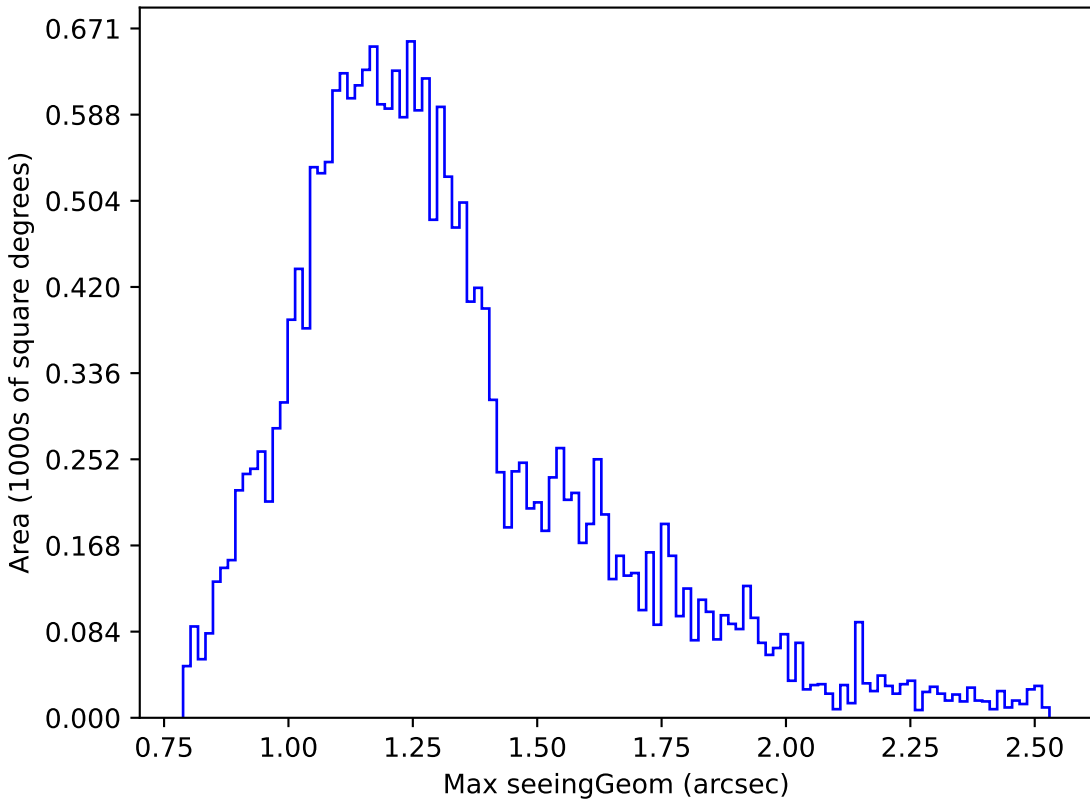
smc_lmc_v3.3_10yrs Yr 1 u band: Max seeingGeom
