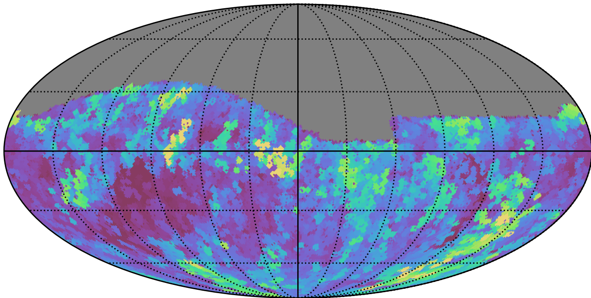
smc_lmc_v3.3_10yrs Yr 1 r band: Max seeingGeom
