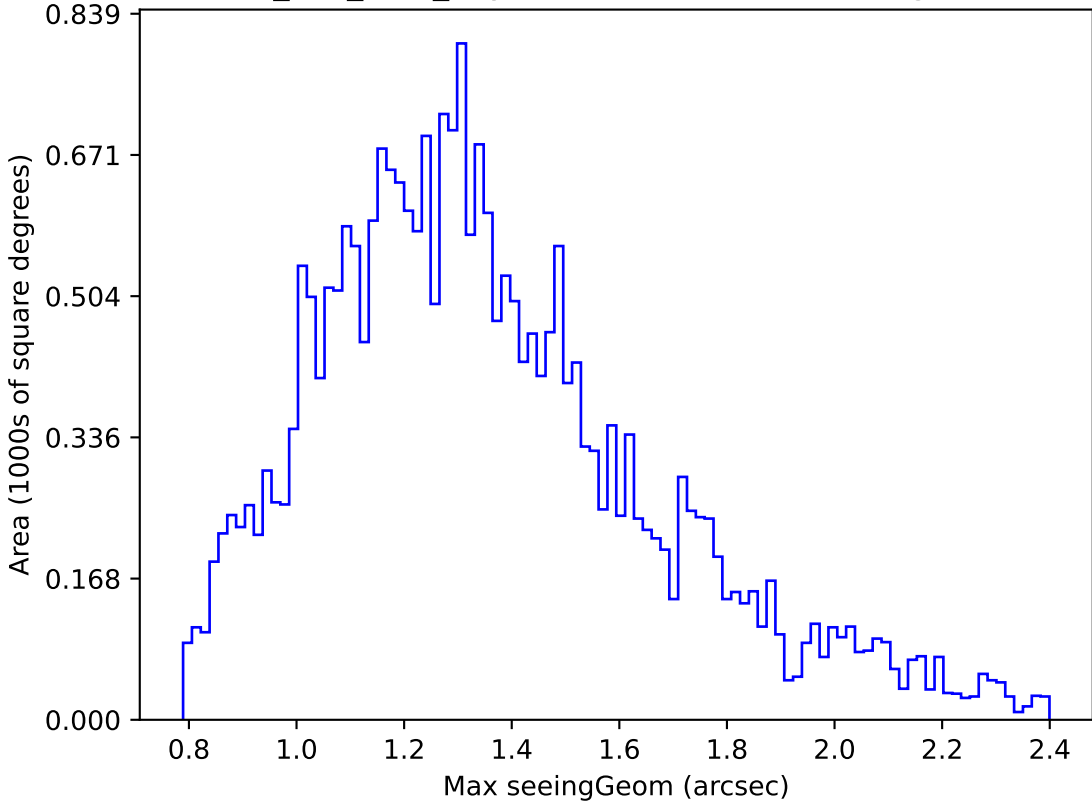
smc_lmc_v3.3_10yrs Yr 1 r band: Max seeingGeom
