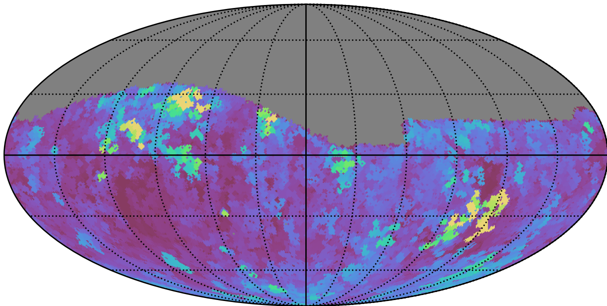
smc_lmc_v3.3_10yrs Yr 1 g band: Max seeingGeom
