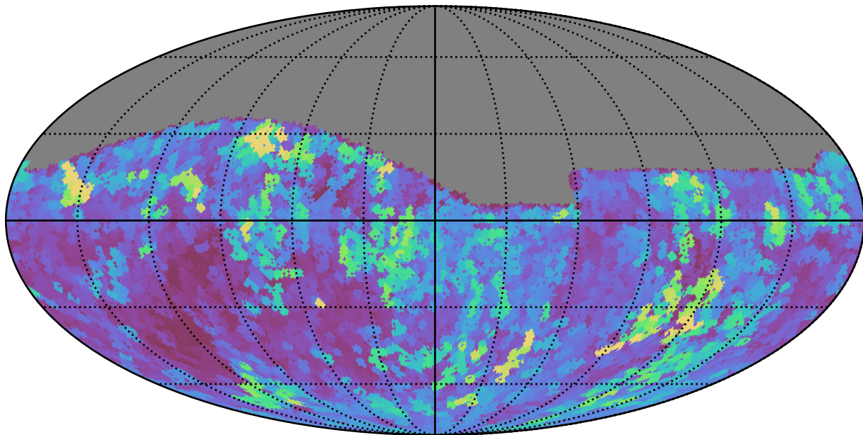
smc_lmc_v3.3_10yrs Yr 1 all bands: Max seeingGeom
