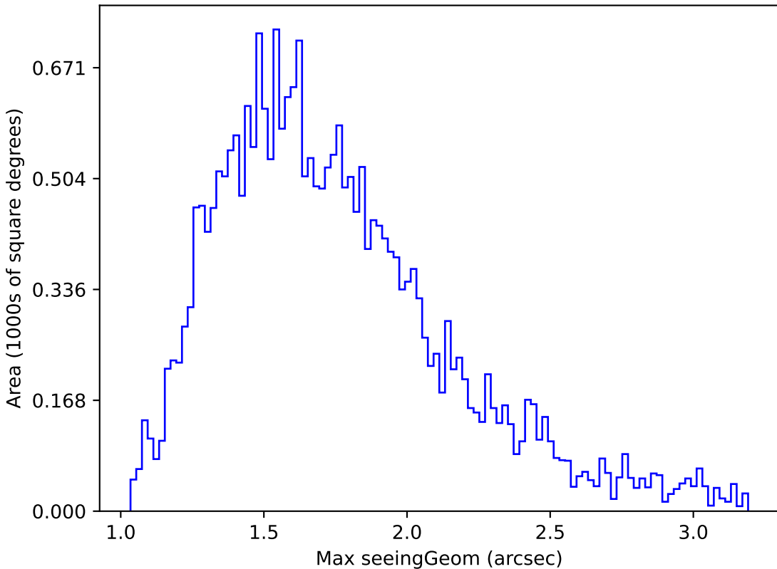
smc_lmc_v3.3_10yrs Yr 1 all bands: Max seeingGeom
