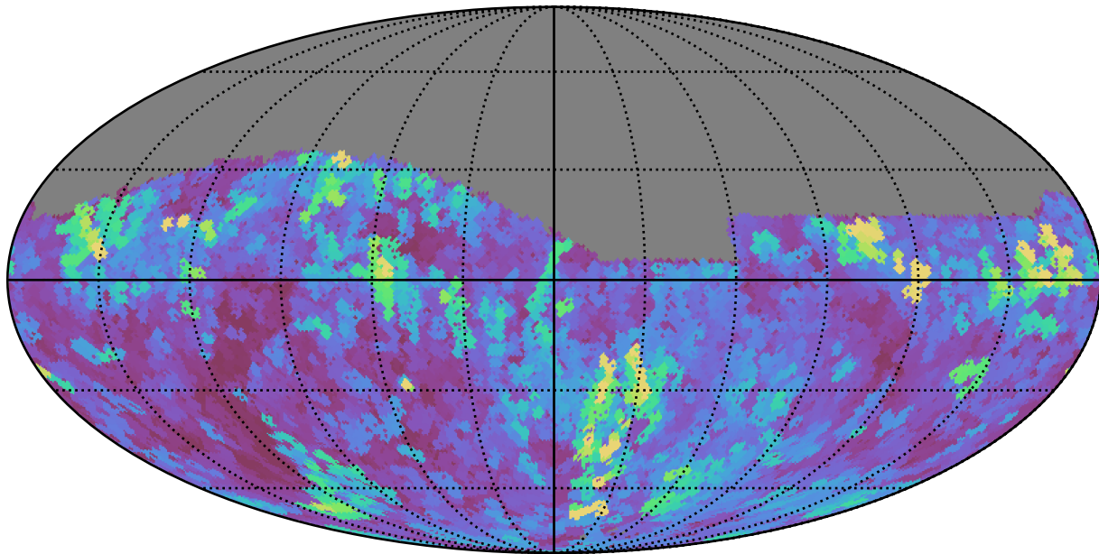
smc_lmc_v3.3_10yrs Yr 1 z band: Max seeingEff
