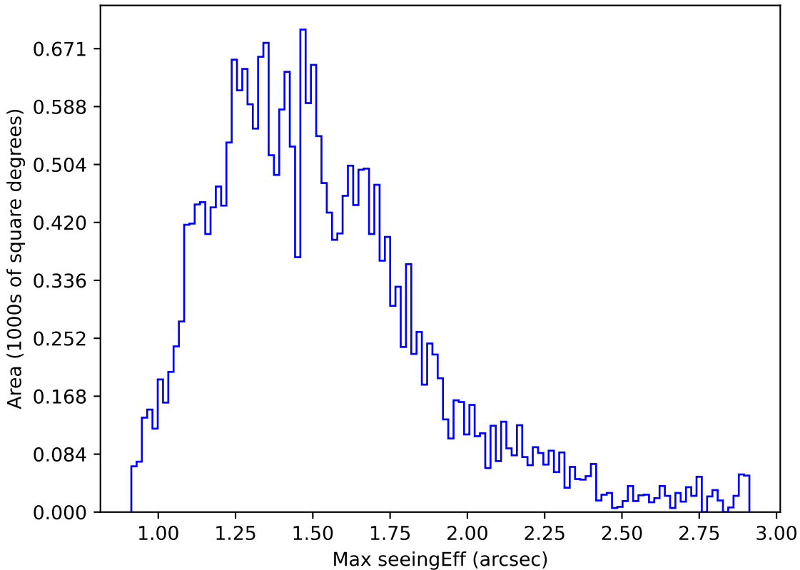
smc_lmc_v3.3_10yrs Yr 1 z band: Max seeingEff
