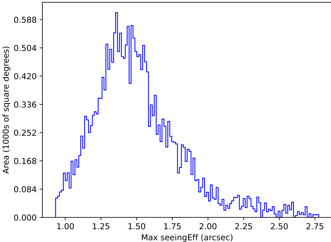
smc_lmc_v3.3_10yrs Yr 1 y band: Max seeingEff
