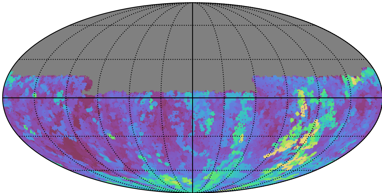
smc_lmc_v3.3_10yrs Yr 1 u band: Max seeingEff
