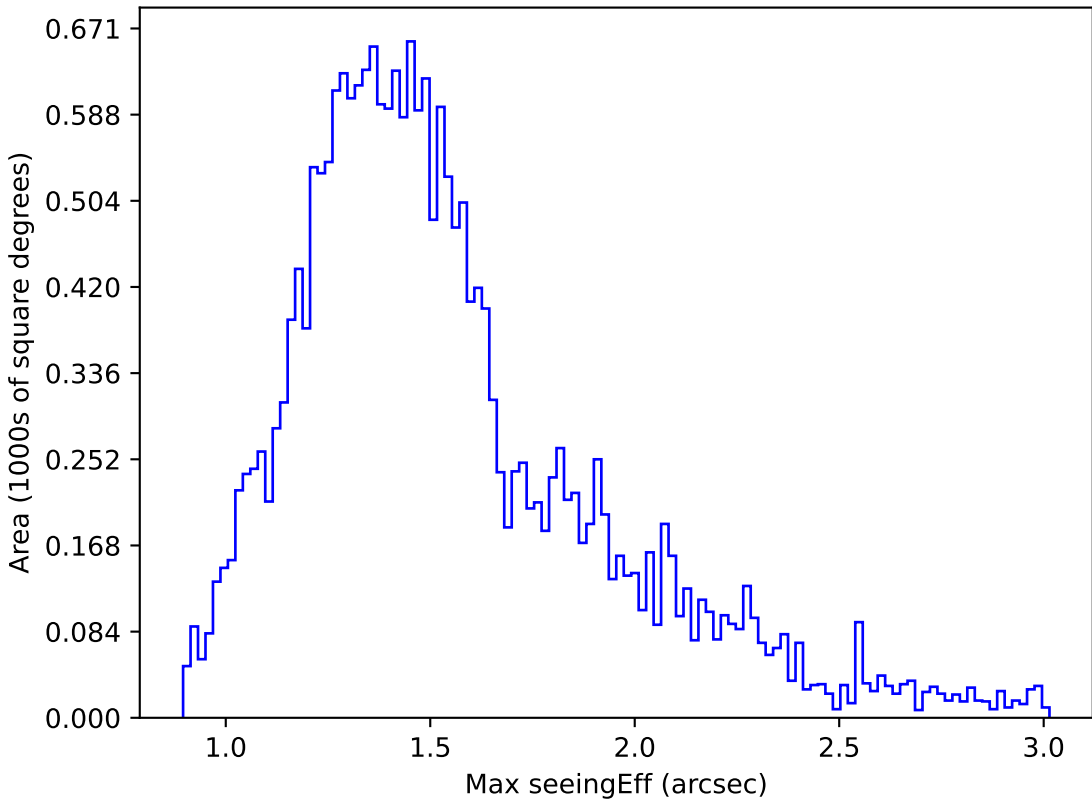
smc_lmc_v3.3_10yrs Yr 1 u band: Max seeingEff
